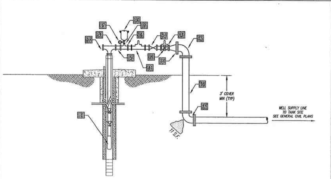
A W-2 TYPICAL WELLHEAD - SECTION VIEW SCALE 1" = 2'
