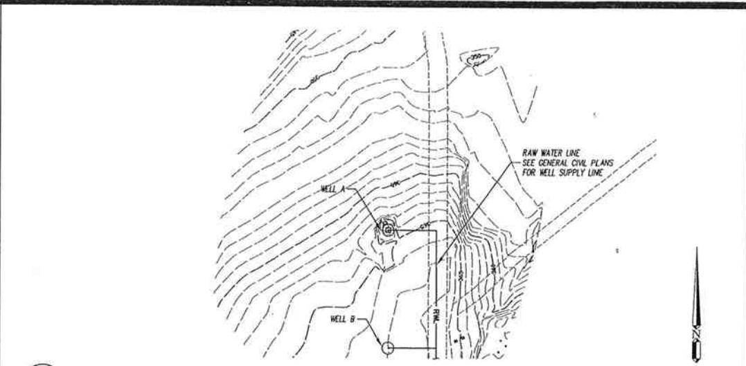
1 W-2 LOCATION OF WELLHEADS A & B SCALE 1" = 50'
