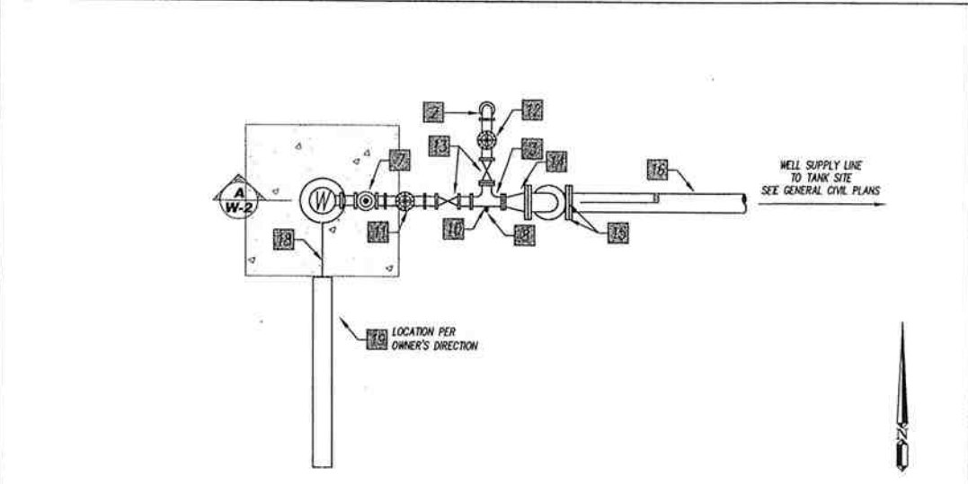
2 W-2 TYPICAL WELLHEAD - PLAN VIEW SCALE 1" = 2'
