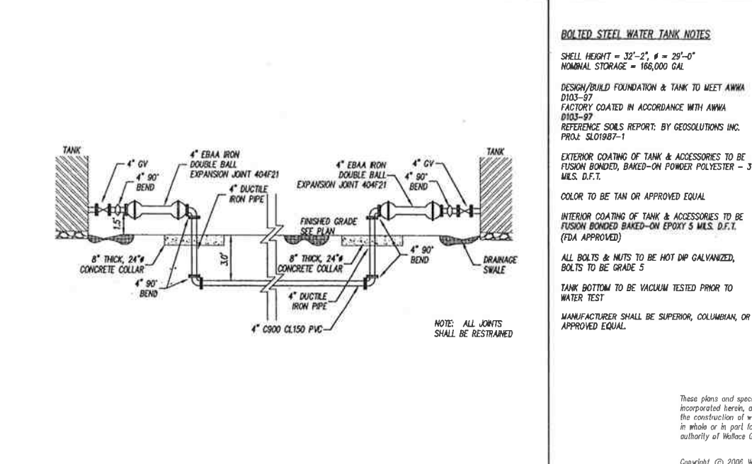
7 W-4 TANK EQUALIZATION PIPE NTS
